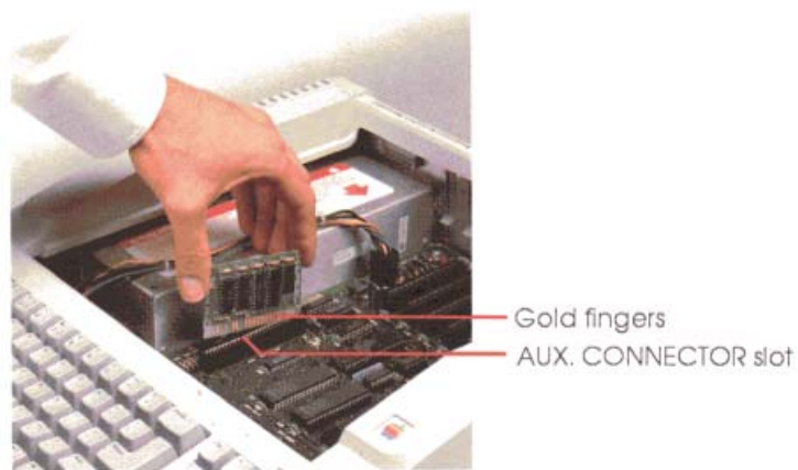
Figure 1-6 Removing the Extended 80-Column Text Card
