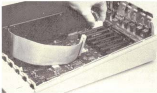
Plug Internal Cord Into Motherboard
