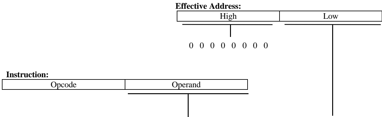
Figure 7-3 Zero Page Addressing.
