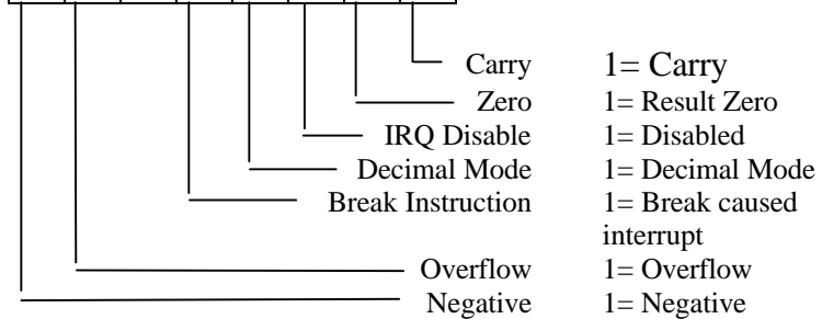
Figure 17-1 6502/65C02 Programming Model
