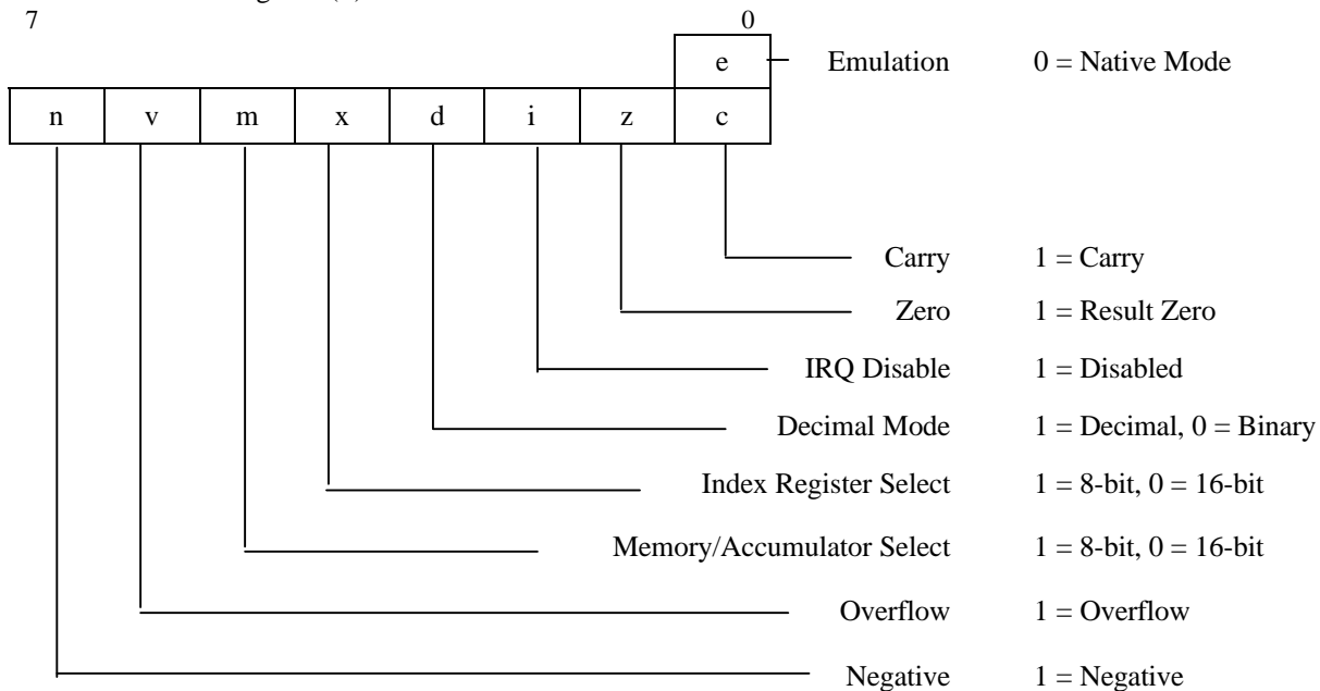
Figure 4-3 65802 Native Mode Programming Model
